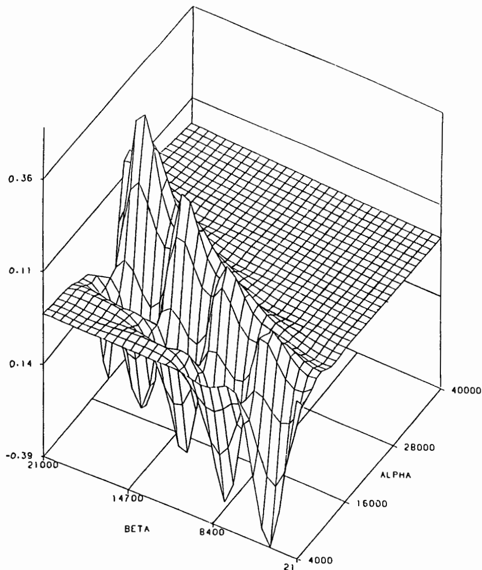
FIGURE 2. Surface of R_{CV}(\alpha, \beta) .
