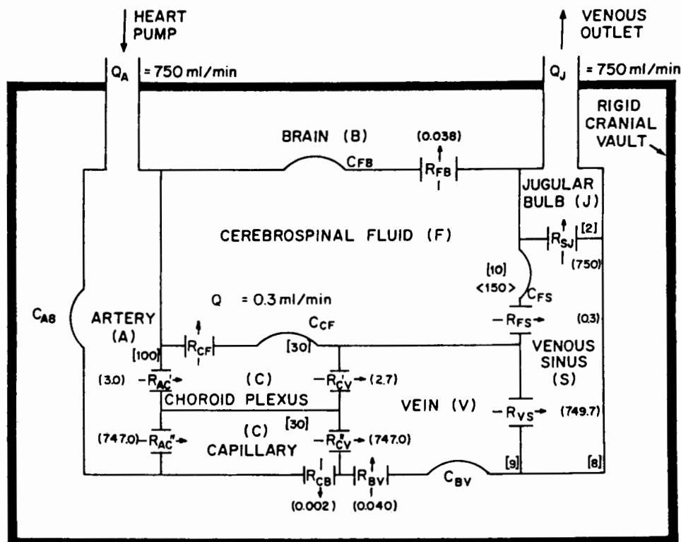
FIGURE 1. Lumped parameter, seven-compartmental fluid system ( R -resistance, C -compliance; [ ] pressure (mm Hg); ( ) flow (ml/min); < > volume (ml)).
